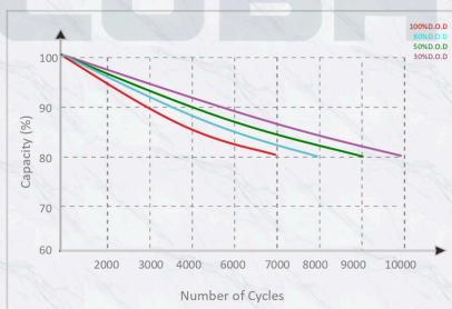
DoD VS Cycle Life (0.2C 25°C)
